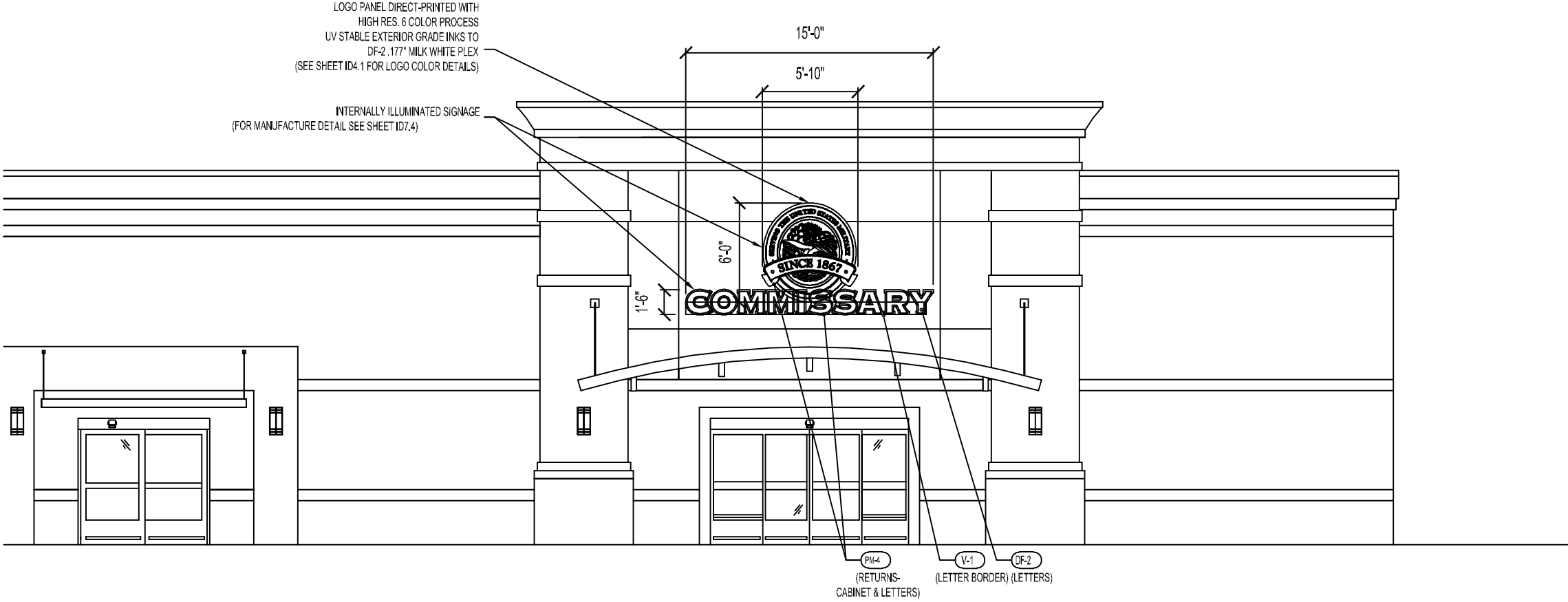
ENTRANCE ELEVATION 1/8"=1'-0"
